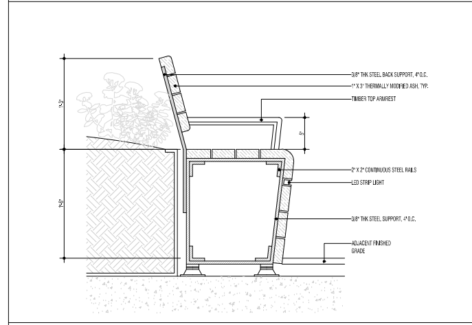
08 TIMBER BENCH, TYP. 1/12" = 1'-0"
