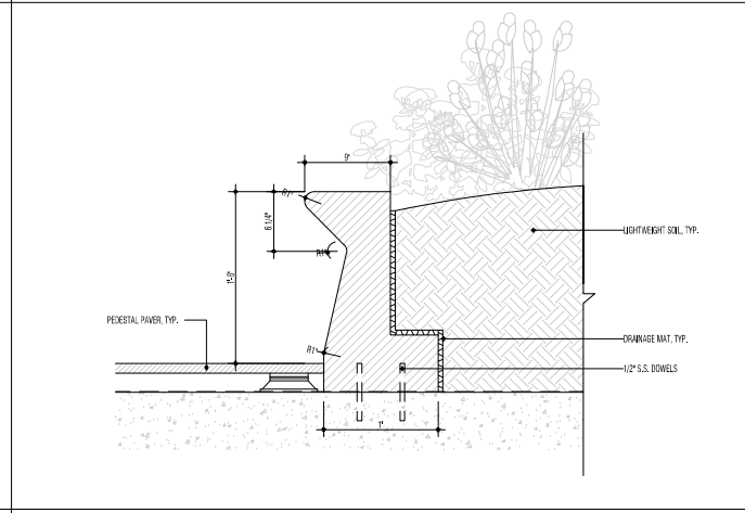
05 PRECAST PLANTER 1/12" = 1'-0"
