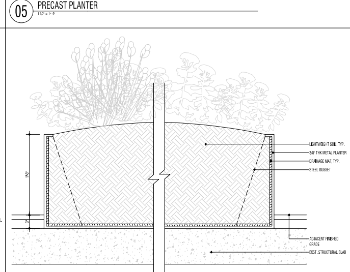
04 METAL PLANTER 1/12" = 1'-0"
