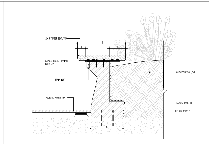
06 BENCH AT PRECAST PLANTER 1/12" = 1'-0"
