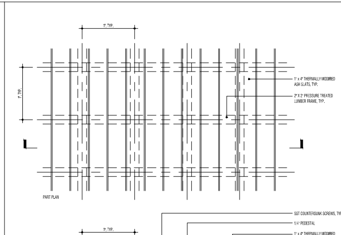
03 TIMBER DECKING 1/12" = 1'-0"
